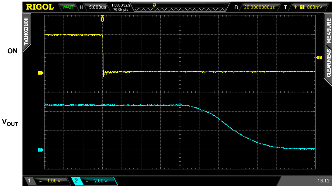
Figure 5. Typical Turn OFF operation waveform for V_{IN} = 4.5\text{ V} , C_{SLEW} = 10\text{ nF} , no C_{LOAD} , R_{LOAD} = 100\ \Omega
