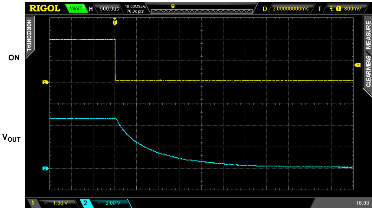
Figure 6. Typical Turn OFF operation waveform for V_{IN} = 4.5\text{ V} , C_{SLEW} = 10\text{ nF} , C_{LOAD} = 10\ \mu\text{F} , R_{LOAD} = 100\ \Omega
